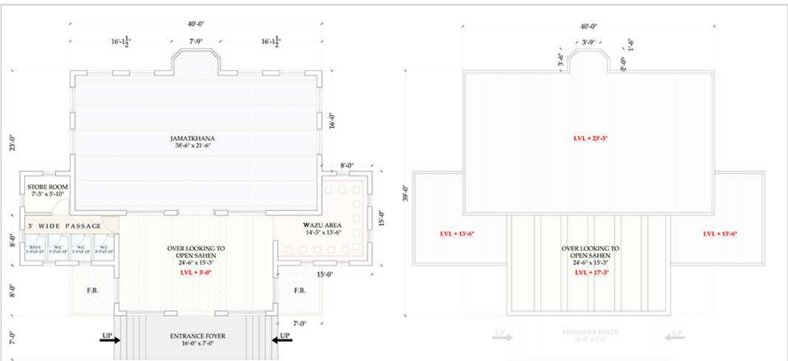
GROUND FLOOR PLAN (1983 SQ.FT. -47 LAKHS)
