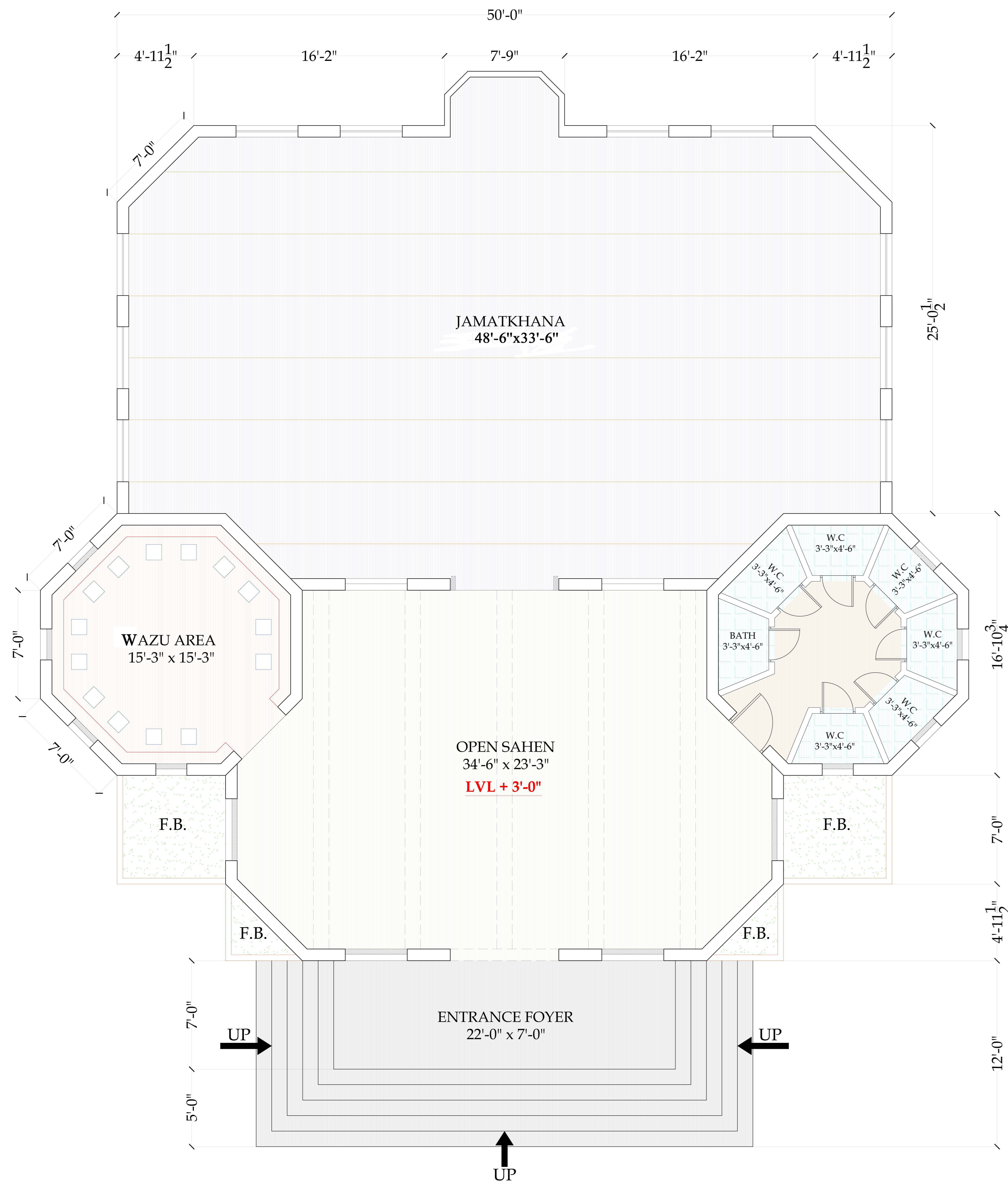
GROUND FLOOR PLAN (3241.58 SQ.FT. -75 LAKHS)
