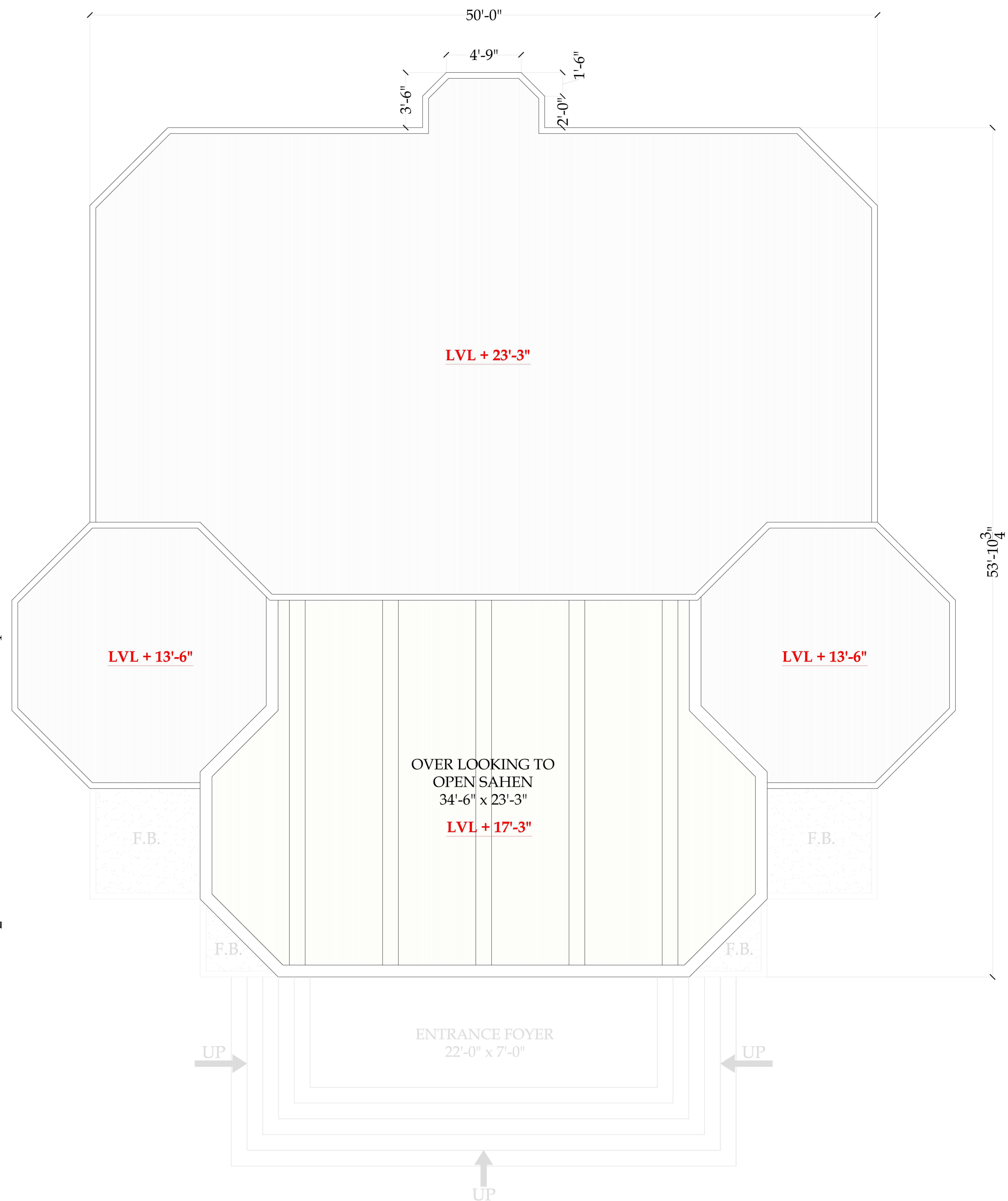
TERRACE FLOOR PLAN
